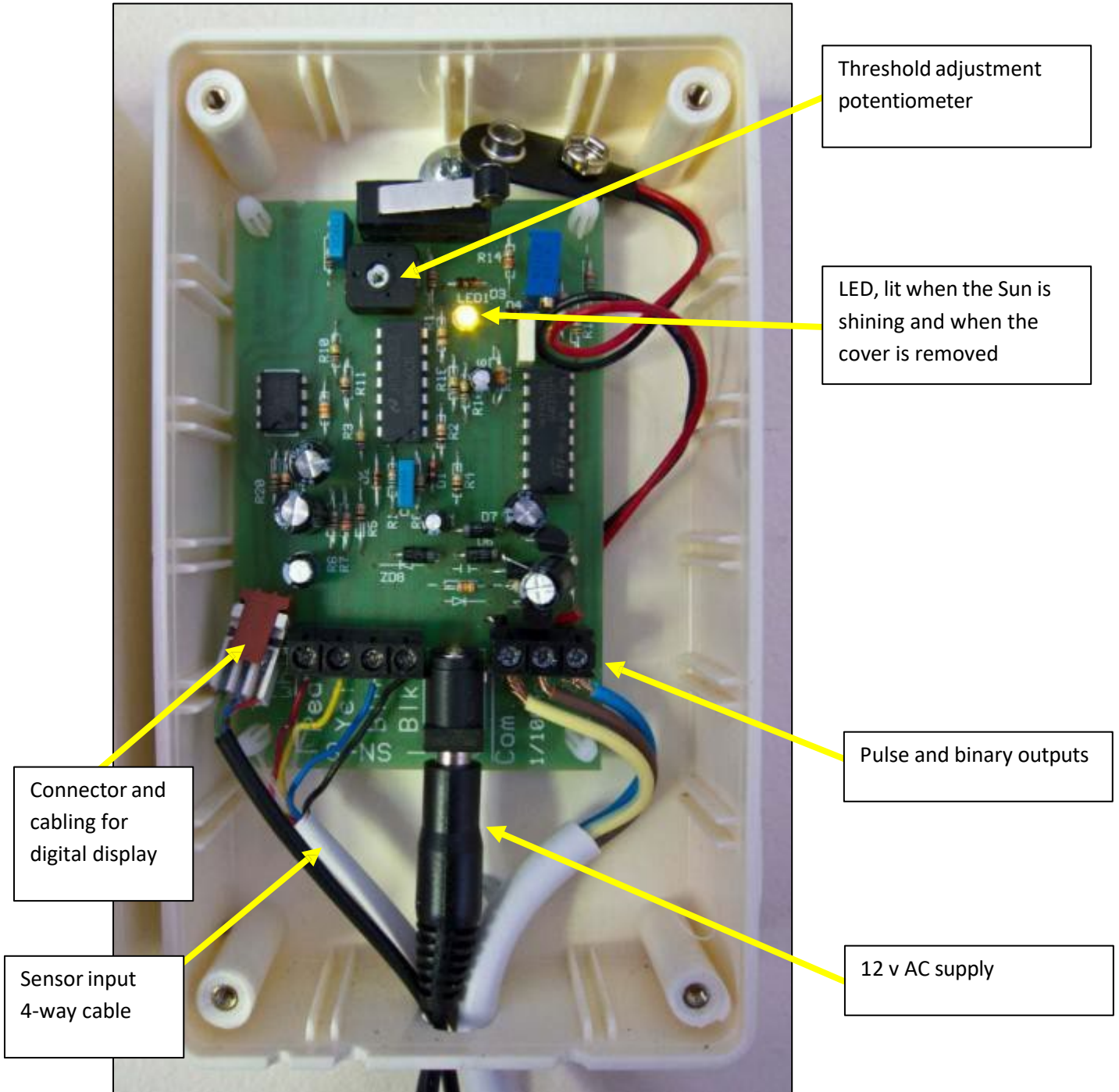
Figure 2 The Instromet sunshine sensor electronics module. Note that the cable used here for the pulse and binary outputs is standard mains cable, but it is NOT carrying mains voltages
