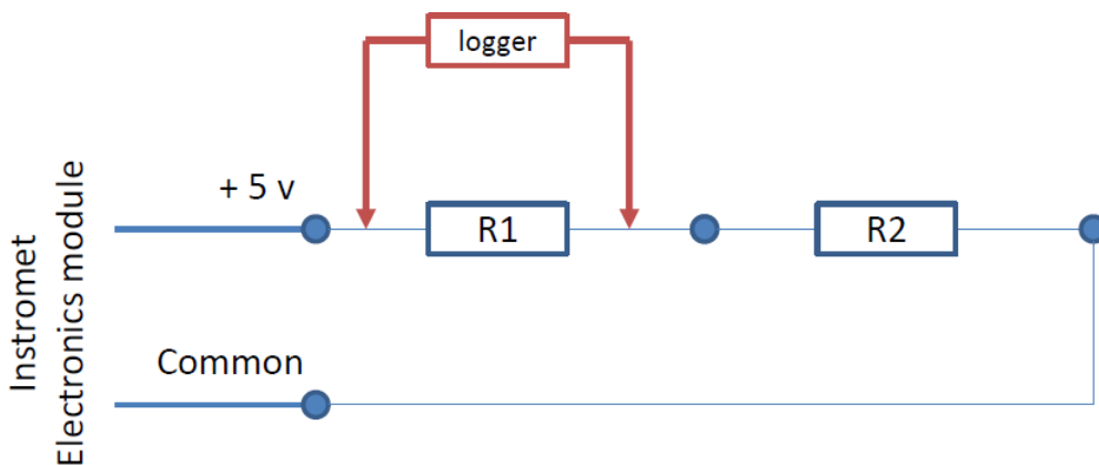
Figure 3 A suitable voltage divider circuit to reduce the binary output to ~ 1.6 v across the logger. R1 = 2.2\text{ k}\Omega , R2 = 4.7\text{ k}\Omega
